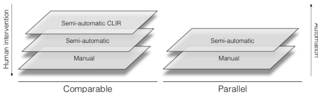
Figure 1: iCompileCorpora layered model.
